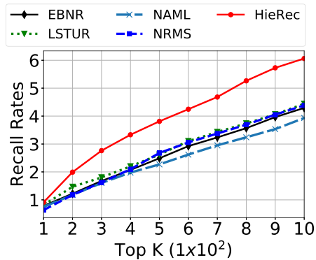
Figure 6: Recall rates of different methods.
