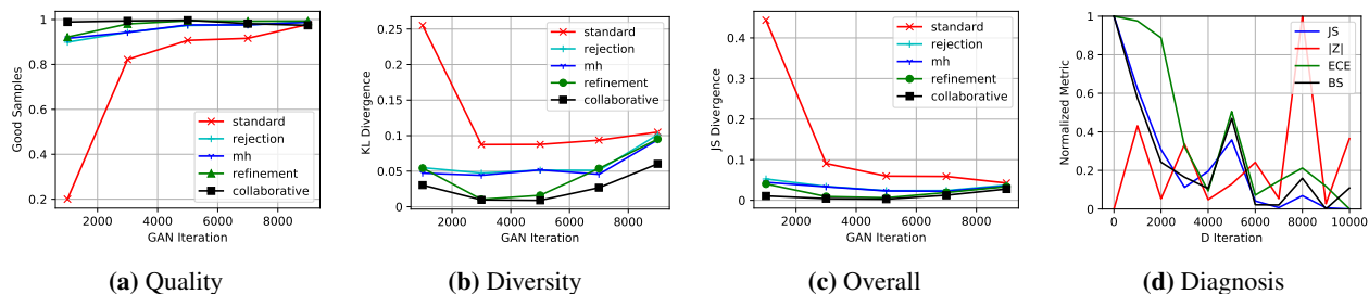
Figure 4: Quantitative results on the imbalanced mixture of eight Gaussians. Evaluated on 10000 samples. ( a ) Proportion of good samples. Higher is better. ( b ) KL divergence between the categorical distribution of real samples and that of good generated samples. Lower is better. ( c ) JS divergence between the augmented categorical distribution of real samples and that of all generated samples. Lower is better. ( d ) The scores of diagnostic metrics and the performance gain from the rejection step at different stages of the discriminator. We apply the MH method to the generator at 1k and normalize the results on each metric to [0,1] for comparison. Among the three diagnostic metrics, the evolution of the Brier Score exhibits the strongest similarity to that of the JS divergence.
