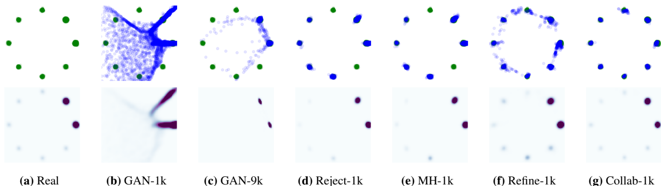
Figure 3: Qualitative evaluation of collaborative sampling in GANs on a synthetic imbalanced mixture of eight Gaussians ( green ). We draw 10k samples ( first row ) from different models and visualize the resulting model distribution using kernel density estimation (KDE) ( second row ). The output samples ( blue ) from the generator at an early stage of training are not of good quality ( b ), whereas training GANs longer results in mode collapse ( c ). Our sample refinement method ( f ) applied to the early terminated GAN not only shifts the proposed samples closer to the real Gaussian components but also expands the categorical coverage. By incorporating the rejection step, ( g ) the full version of our collaborative sampling scheme succeeds in recovering all modes without compromising sample quality, significantly outperforming ( d ) the rejection sampling (Azadi et al. 2019) and ( e ) the Metropolis-Hastings (MH) algorithm with independence sampler (Turner et al. 2019).
