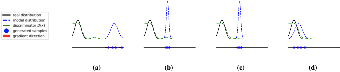
Figure 2: Illustration of our collaborative sampling scheme with discriminator shaping. (a) The trained generator implicitly provides a model distribution that is close to, but not identical to, the real data distribution. At this stage, the gradient provided by the discriminator suggests informed moves. (b) However, the loss landscape from the discriminator may present local optima, hence the sample refinement process ceases. (c) Our discriminator shaping method uses the refined samples to smoothen the loss landscape. (d) The shaped loss landscape is able to better guide the refinement process, shifting the model distribution closer to the target.
