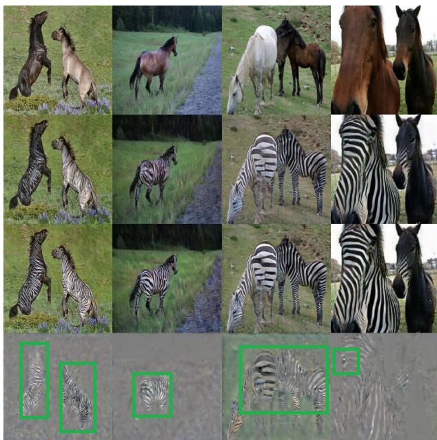
Figure 8: Results of our collaborative sampling scheme in CycleGAN for unpaired image-to-image translation at 256 \times 256 resolution. The real horse images (top) are translated into synthetic zebra images (second row), which are further refined by our method (third row). The differences between the translated and refined images are concentrated on zebra patterns (bottom).
