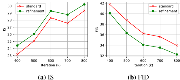
Figure 7: Quantitative comparison between our collaborative sampling scheme and the standard sampling for SAGAN on ImageNet (Batch size 16). Higher is better for IS and lower is better for FID.
