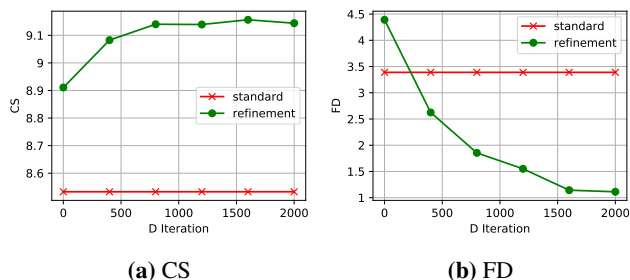
Figure 10: Quantitative effect of discriminator shaping. We apply our sample refinement method using discriminators shaped for different iterations. Higher is better for CS and lower is better for FD.
